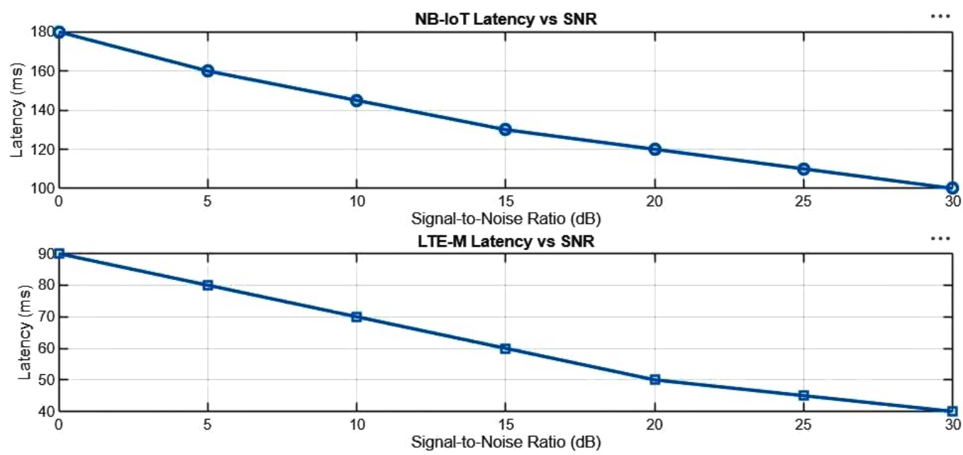
Command Window
